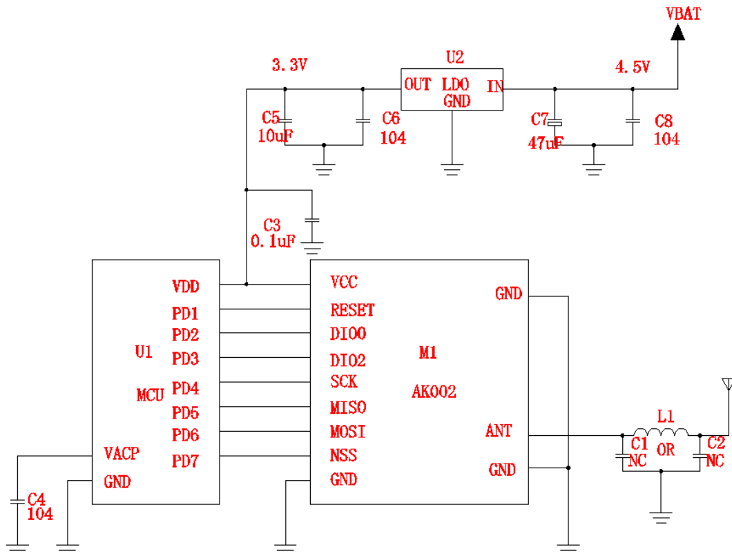
Figure 34 Typical Application Schematic
