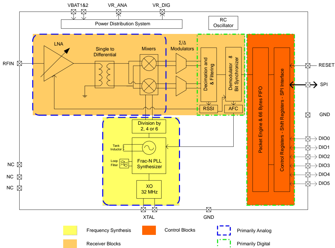
Figure 1. Block Diagram
