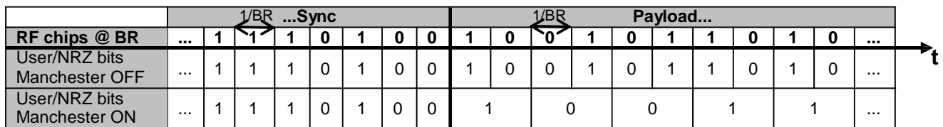
Figure 30 Manchester Decoding
