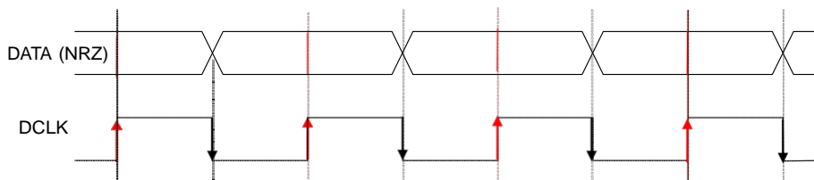
Figure 24. Rx Processing in Continuous Mode
