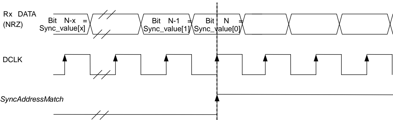
Figure 22. Sync Word Recognition
