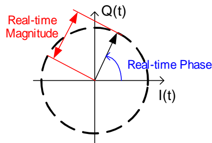
Figure 6. Cordic Extraction
