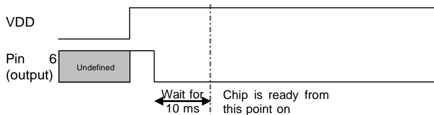
Figure 32 POR Timing Diagram
