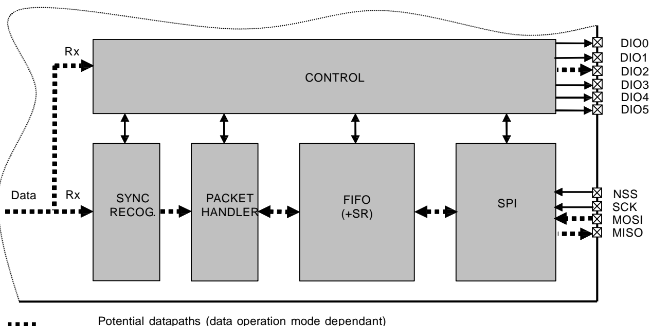
Figure 18. AK002 Data Processing Conceptual View
