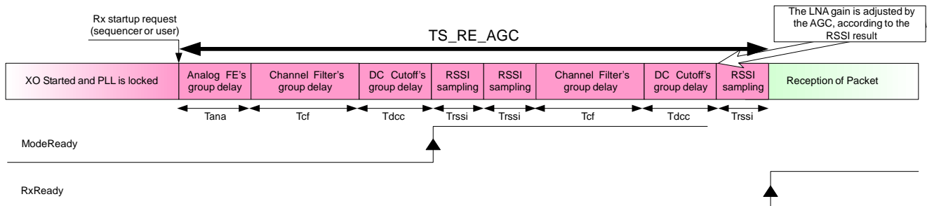
Figure 13. Rx Startup - AGC, no AFC
