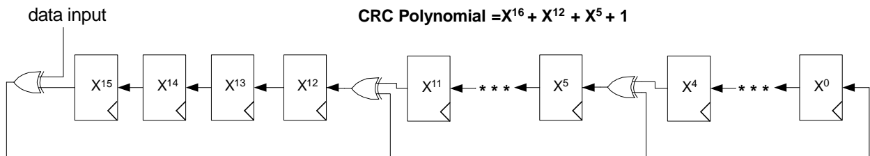
Figure 29. RC Implementation
