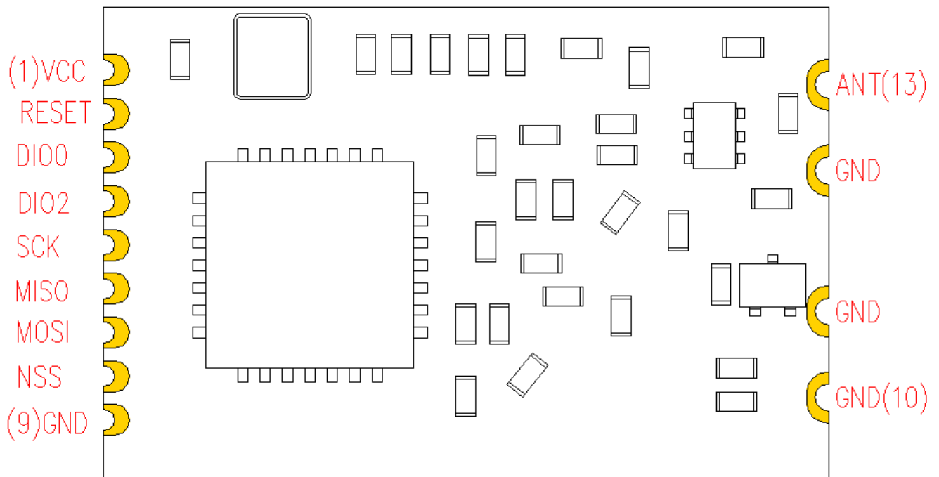
Figure 2. Pin Diagrams
