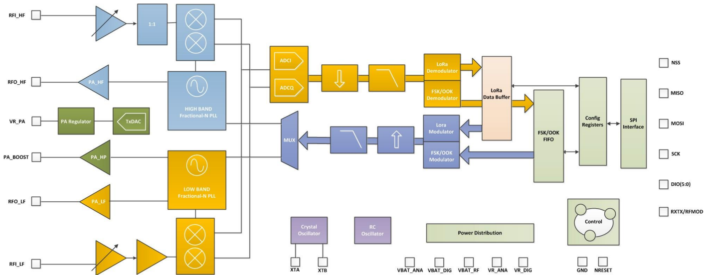
Figure 3. HC1276/77/78 Block Schematic Diagram
