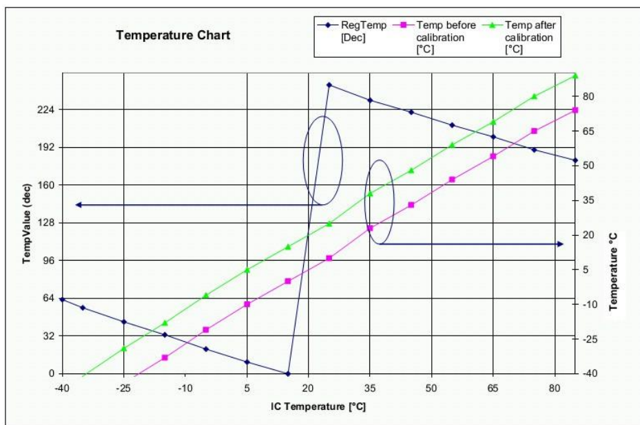
Figure 40. Temperature Sensor Response
