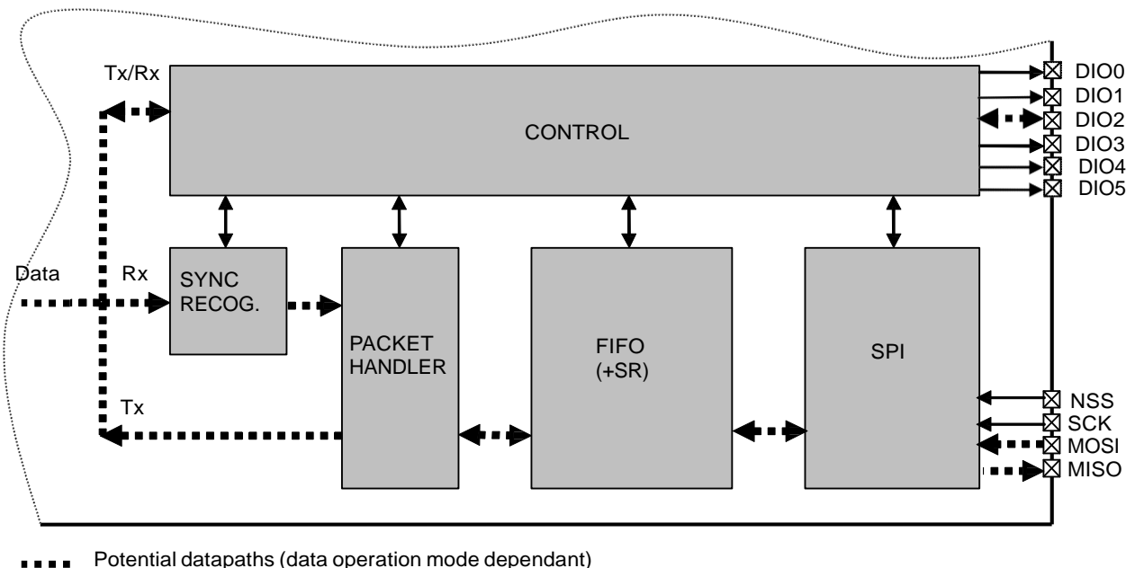
Figure 24. HC1276/77/78 Data Processing Conceptual View
