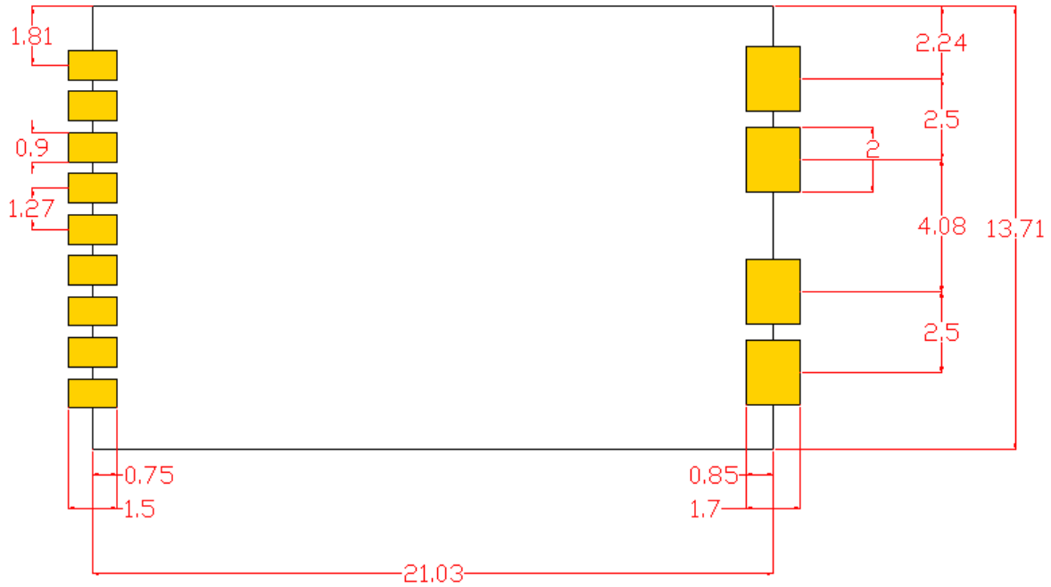
Figure 58. Recommended Land Pattern
