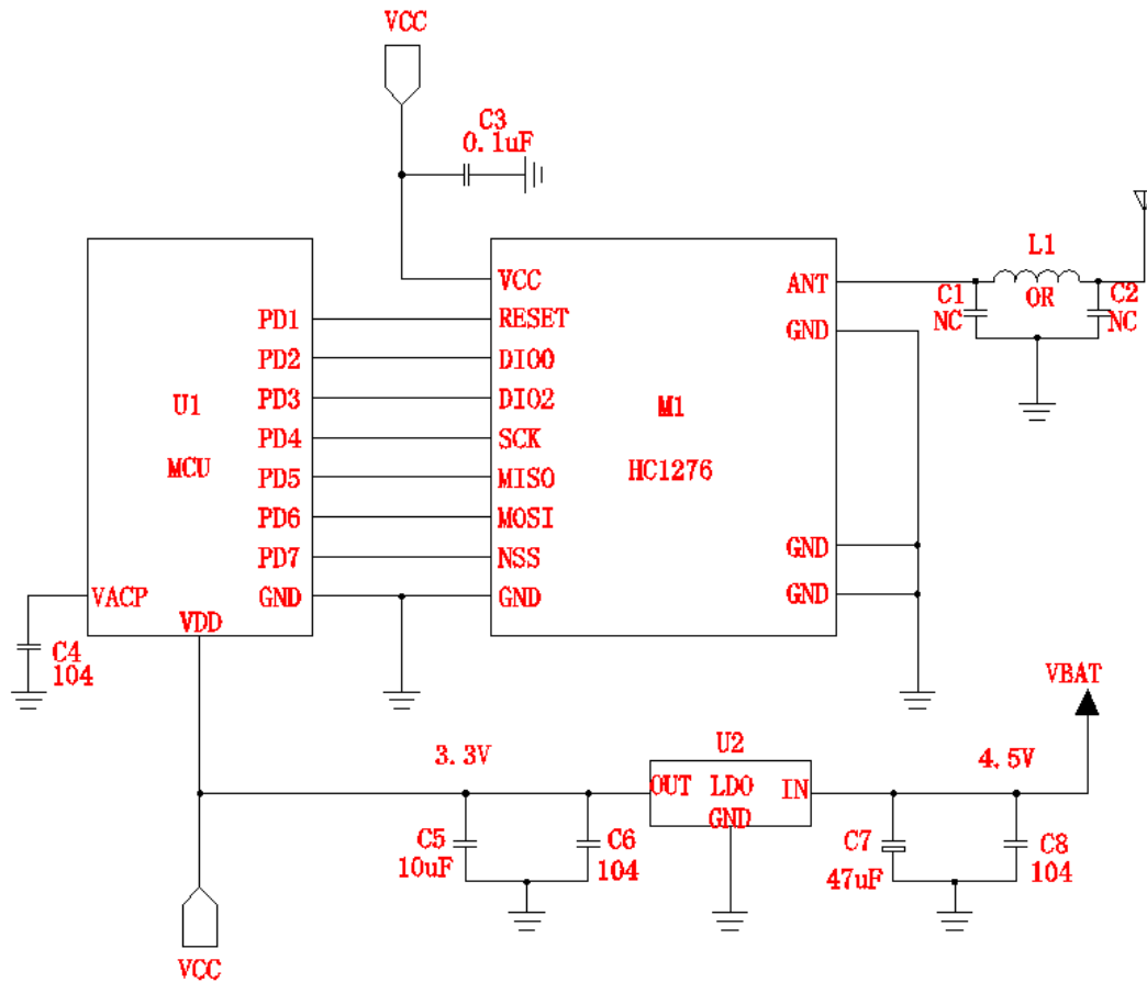
Figure 56 Typical Application Schematic
