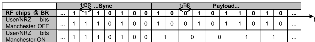
Figure 35. Manchester Encoding/Decoding
