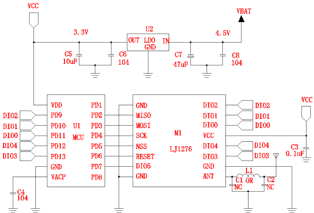
Figure 56 Typical Application Schematic
