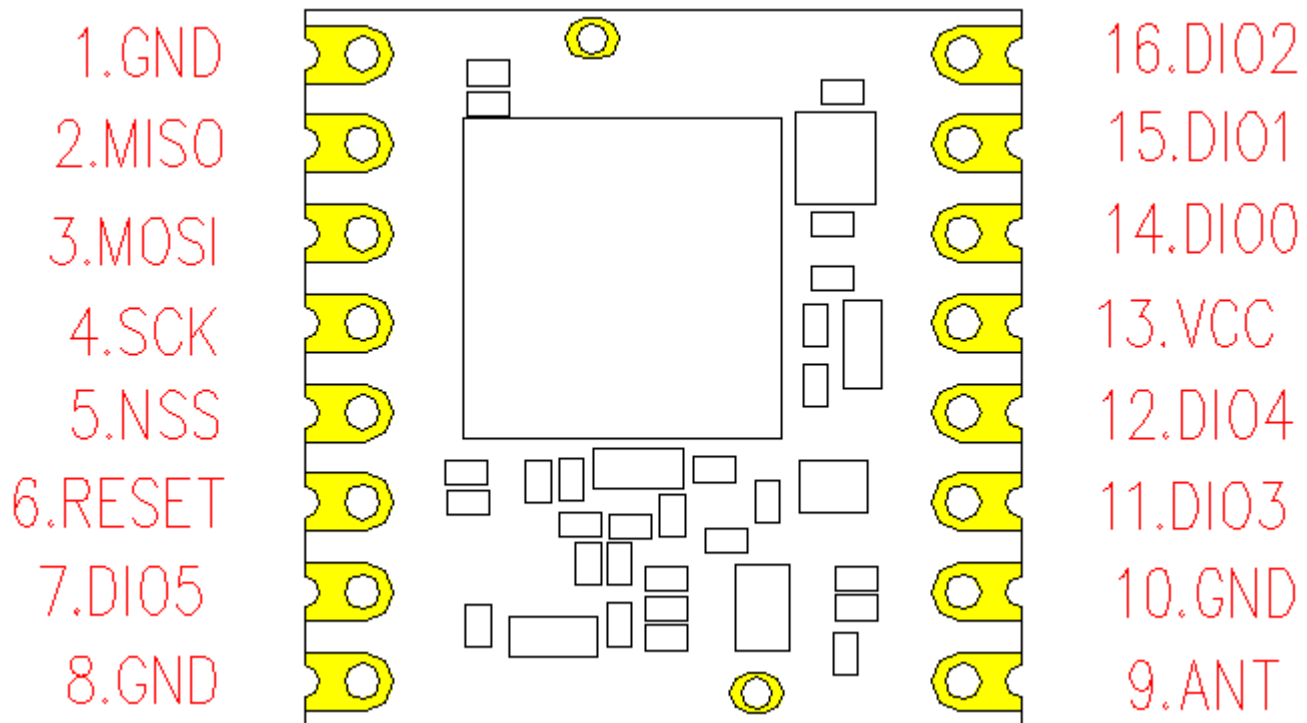
Figure 2. Pin Diagrams
