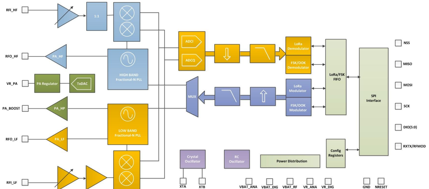
Figure 1. Block Diagram
