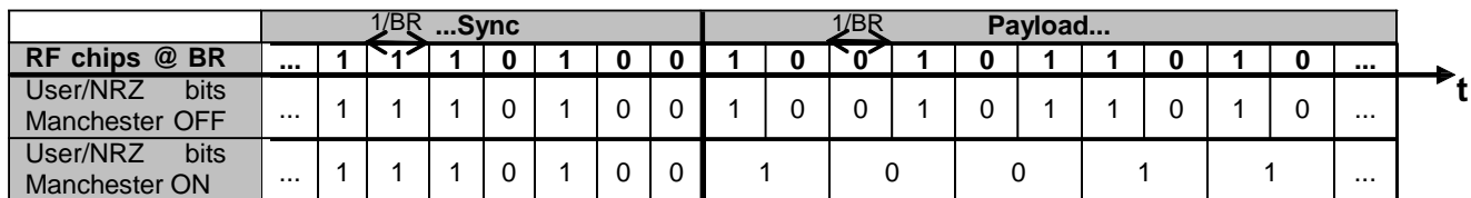
Figure 35. Manchester Encoding/Decoding
