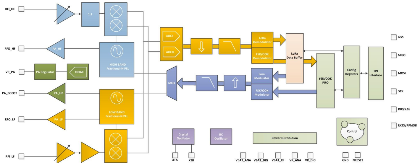
Figure 3. LJ1276/77/78 Block Schematic Diagram
