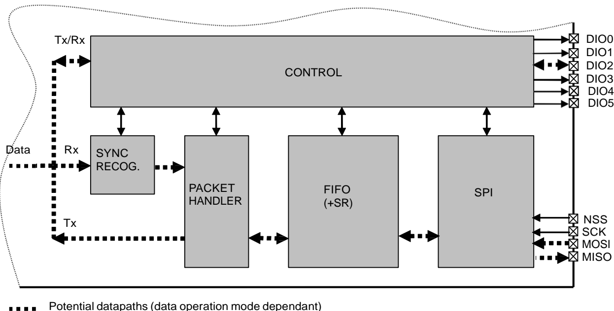
Figure 24. LJ1276/77/78 Data Processing Conceptual View
