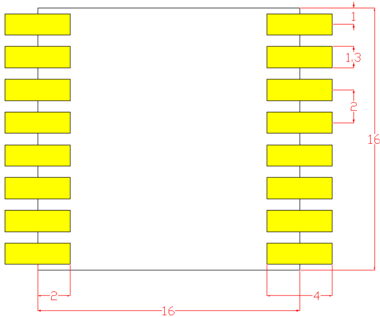
Figure 58. Recommended Land Pattern
